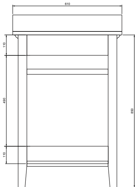
Back View
